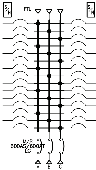
400 A or 600 A PowerPacT L-Frame Main Circuit Breaker with Feed-Thru Lugs
